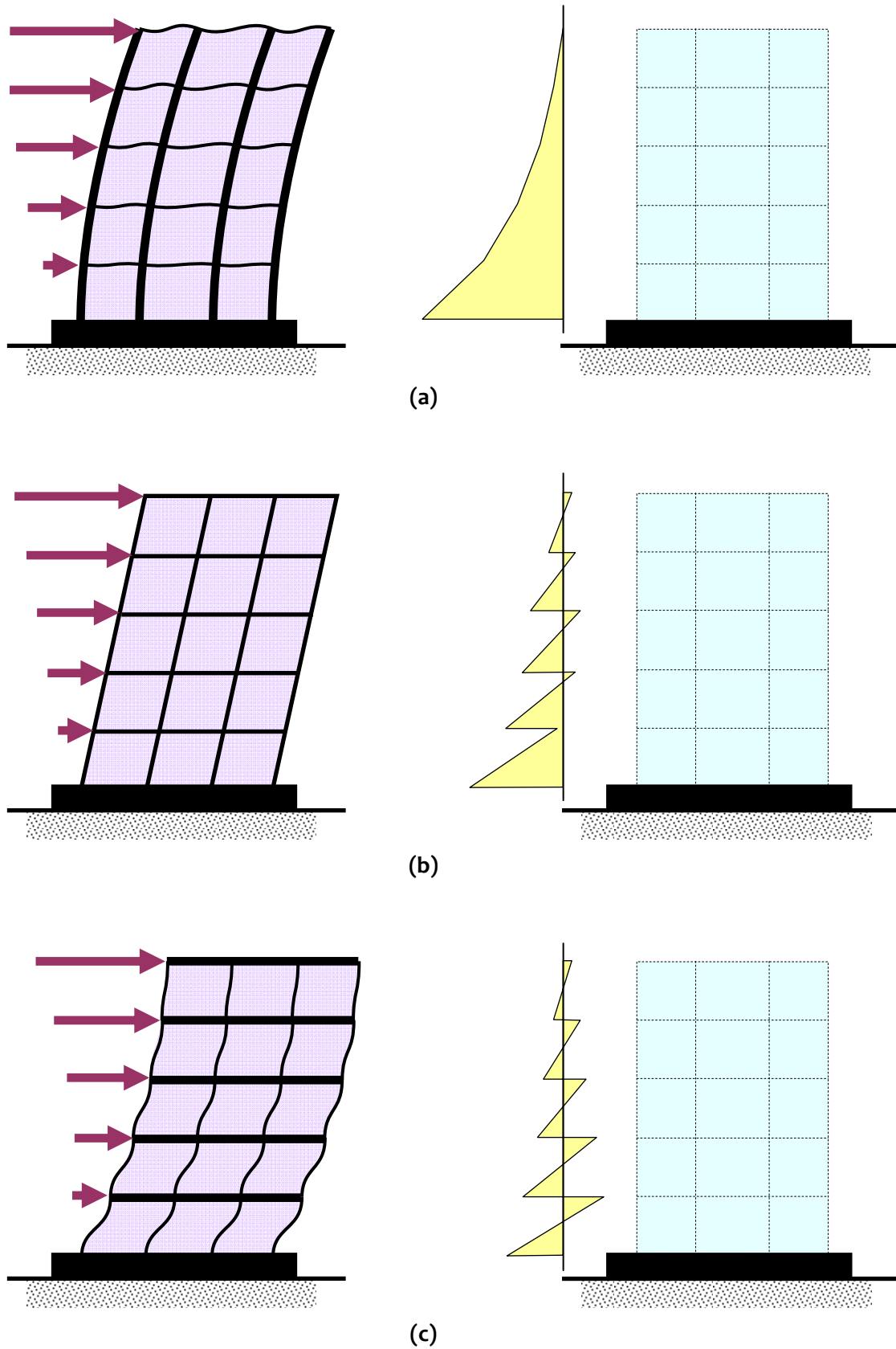
Figure 3.39: Two extreme cases of overall frame action: (a) FLEXURE Deformation Mode: Overall cantilever column action owing to extremely rotationally flexible beams ( I_c/I_b \rightarrow \infty ), (b) INTERMEDIATE Deformation Mode: Combined column-beam action owing to reasonably close rotationally flexible columns and beams, and (c) SHEAR Deformation Mode: Double-curvature column action owing to extremely rotationally stiff beams ( I_c/I_b \rightarrow 0 )
