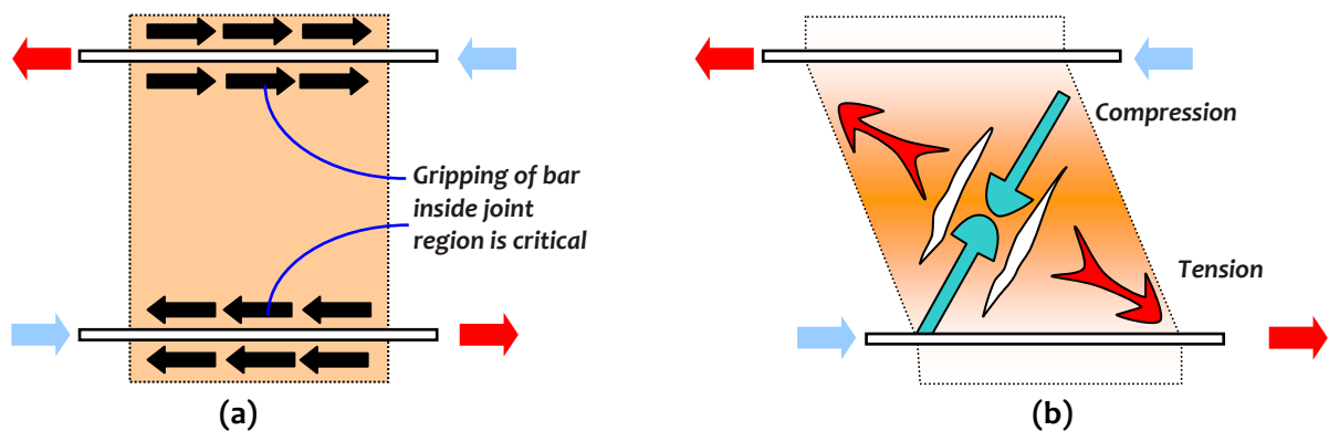
Figure 4.10: Beam-Column Joints in Buildings: (a) Loss of grip on beam bars in joint region; large column width and good concrete help in holding the beam bars, and (b) Distortion of joint: causes diagonal cracking and crushing of concrete
