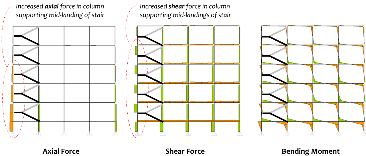
Figure 3.91: Building with staircase: Stair slabs provide intermediate restraints leading to short-column effect
