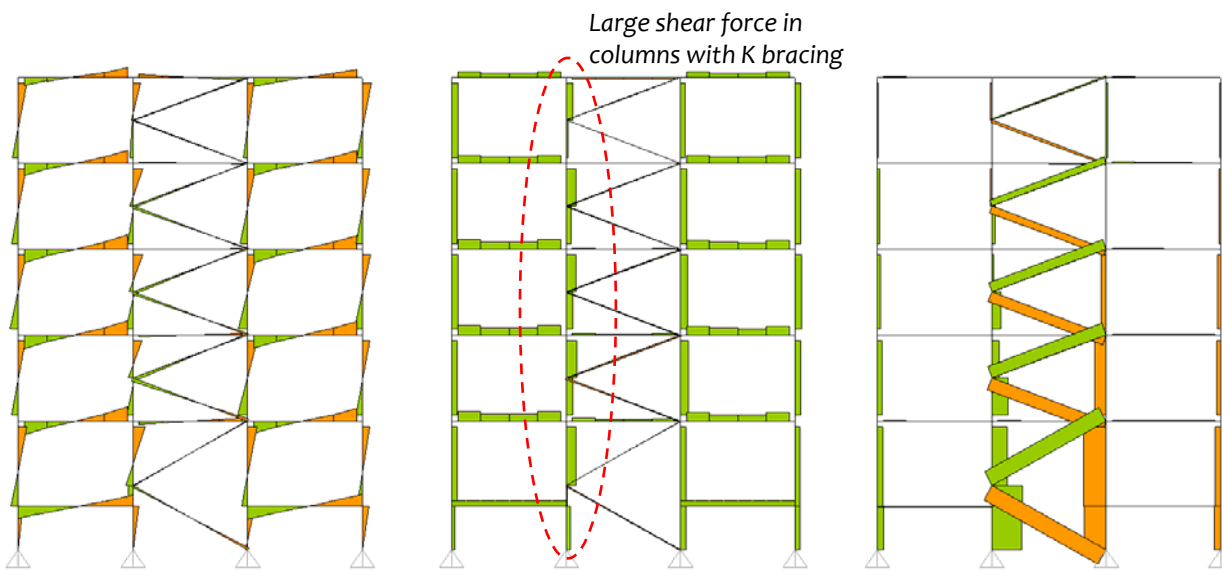
K-BRACES
