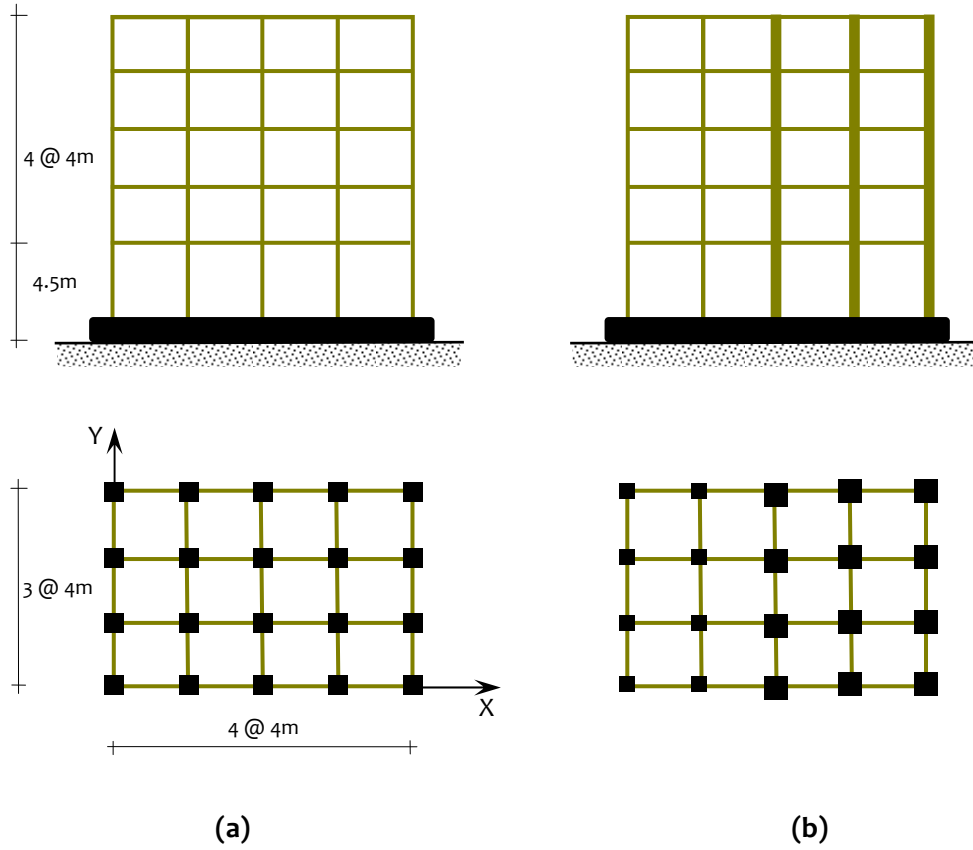
Figure 4.19: Lateral strength asymmetry in plan of building: (a) Benchmark 5-storey building with columns of uniform strength; and (b) Similar 5-storey building, but with asymmetry in column strengths in plan
