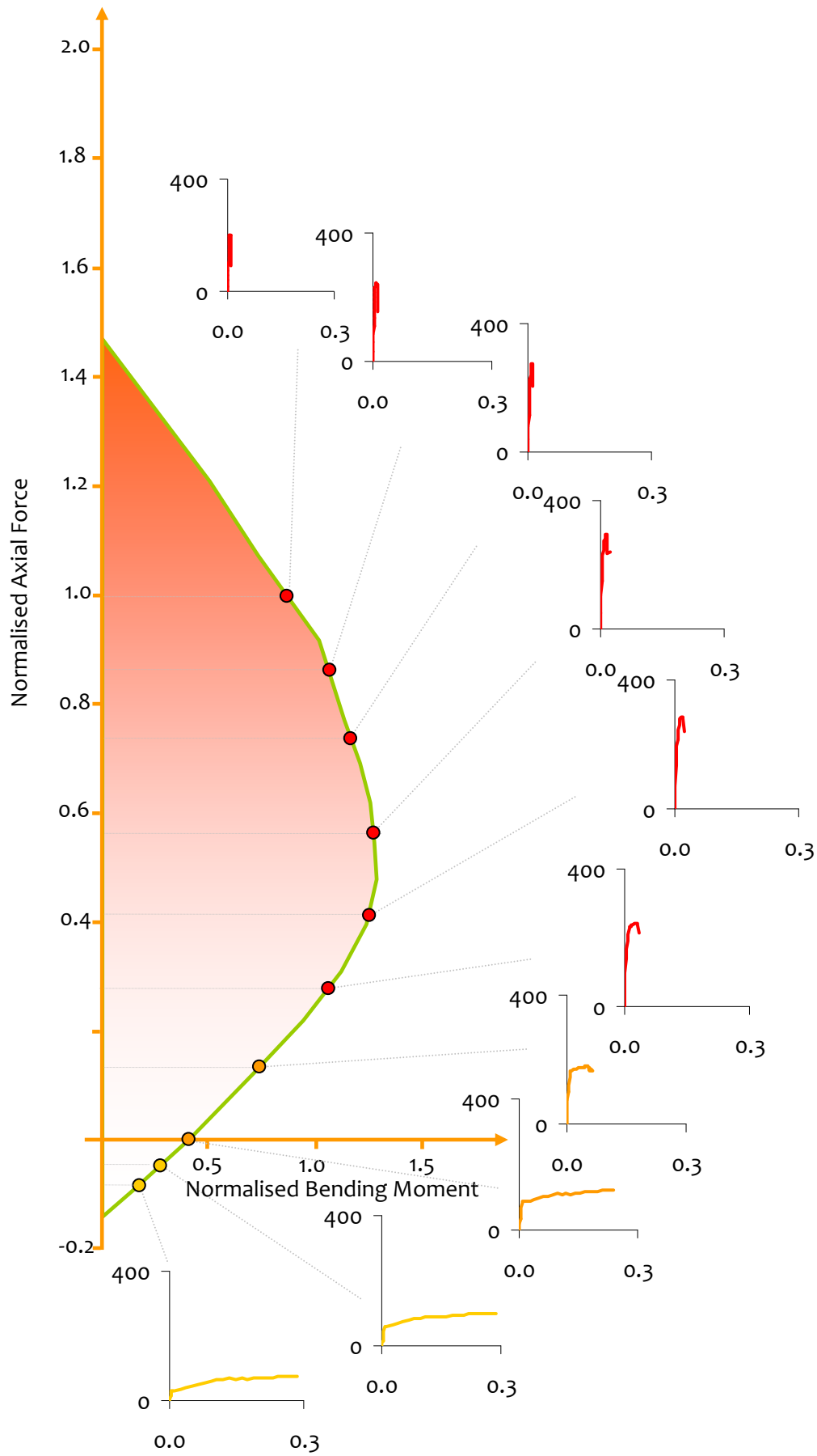
Figure 4.49: ACTUAL P - M interaction envelopes: with UNCONFINED concrete M - \phi relations at different axial loads
