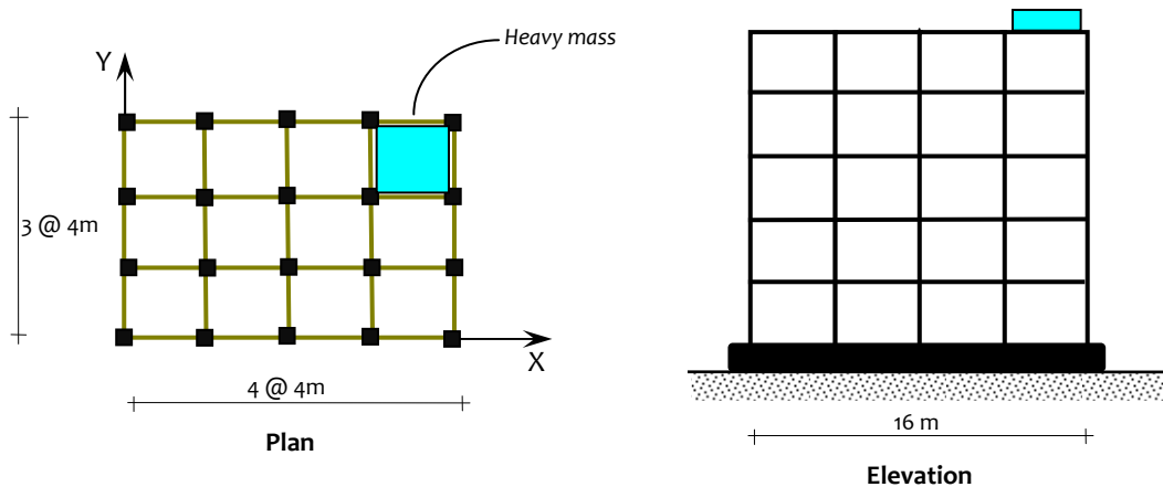
Figure 3.85: Asymmetry of mass in plan: Concentrated mass at one corner of building
