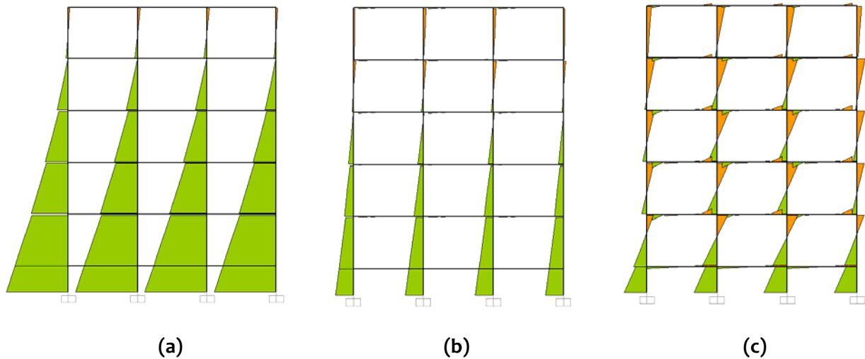
Figure 3.40: Bending moment in members of buildings under lateral load: (a) I_c/I_b = 1000 (Flexure deformation), (b) I_c/I_b = 512 , and (c) I_c/I_b = 7 (Shear deformation)
