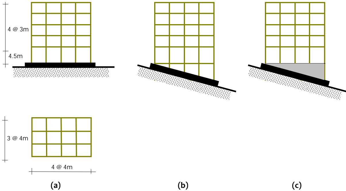
Figure 4.35: Short columns effect in a building: (a) Benchmark 5-storey building with no short columns , (b) Similar 5-storey building with sloping ground ; and (c) Similar 5-storey building with sloping ground but the sloped portion filled with an RC wall in the inclined portion only
