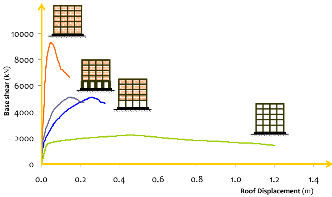
Figure 4.67: Open ground storey building: Influence of infill masonry significant on overall ductility
