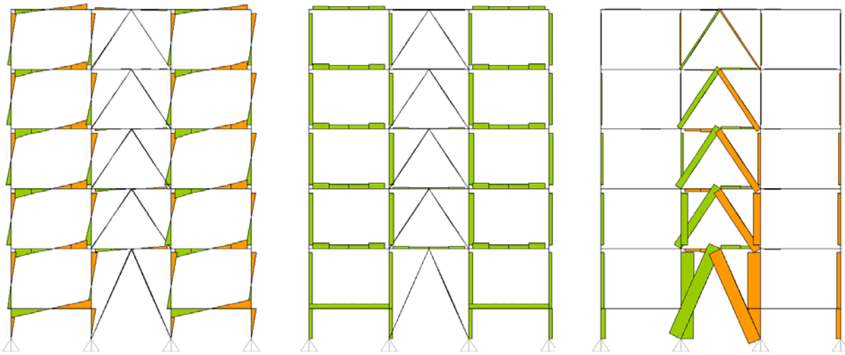
CHEVRON BRACES
