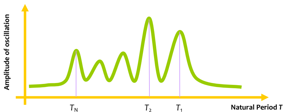
Figure 2.5: Multiple natural periods: Amplitude of oscillation of a building or any of its responses (e.g., bending moments in columns) is amplified when shaken at the natural frequencies
