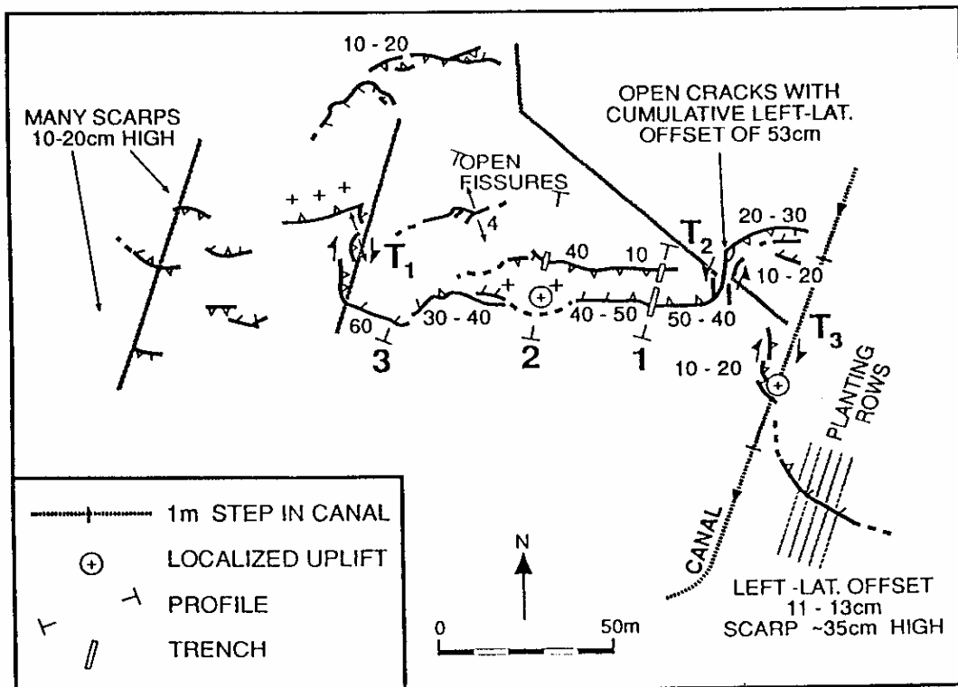
Figure 5b. Detailed map of well-developed and preserved portion of the surface rupture in untilled field. T_1 , T_2 , and T_3 are transfer faults. Trenches 1 and 2 (Figure 9) are along profiles 1 and 2 (Figure 6).
