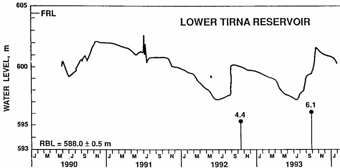
Figure 13. Water level in the lower Tirna reservoir and the timing and magnitudes of the mainshocks in the 1992 and 1993 sequences at Killari (modified from Rastogi [1994]). FRL is full reservoir level; RBL is river bed level.
