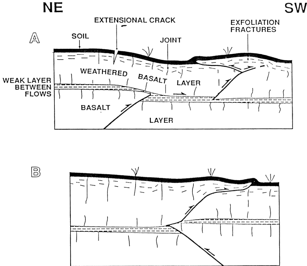
Figure 7. Schematic sections of hypothetical structures at the shallow end of the 1993 fault rupture, which is estimated to dip 46^\circ to the southwest (Figure 3b). This structural complexity is ascribed to interbedded strong and weak layers in the Deccan Traps and probably extends deeper than is shown here. Slip on the horizontal weak layers may be responsible for the double vergence and the complex pattern of surface faulting. Sections A and B are inspired by profiles 2 and 1 (Figure 5b), respectively.
