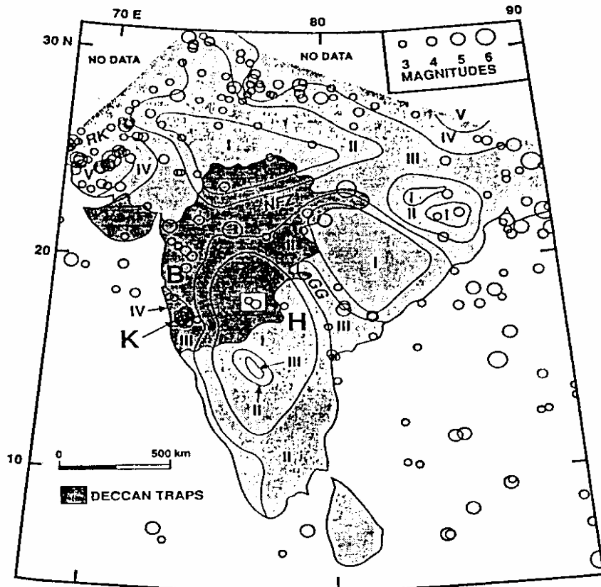
Figure 1. Seismicity map of peninsular India (1900-1992, compiled from Global Hypocenter and Preliminary Epicenter Determination files of the National Earthquake Information Center) and earthquake hazard zones [Krishna, 1992]; hazard increases from I to V. Hazard zonation is based on historic seismicity and on repeatedly deformed structural features, such as the Rann of Kutch (RK), the Narabada fault zone (NFZ), and the Godvari graben (GG). B is Bombay, H is Hyderabad, and K is Koyna. The Killari source (unshaded box) is in the southeastern part of the Deccan Traps (dark shading) and is marked by two epicenters ( M=4.4 and M=3.9 ) from the precursory burst of felt earthquakes in 1992.
