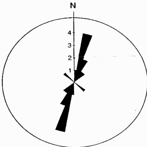
Figure 11. Strike distribution of 10 subvertical joints (all with dip angles \geq 80^\circ ) in trench 1S.
