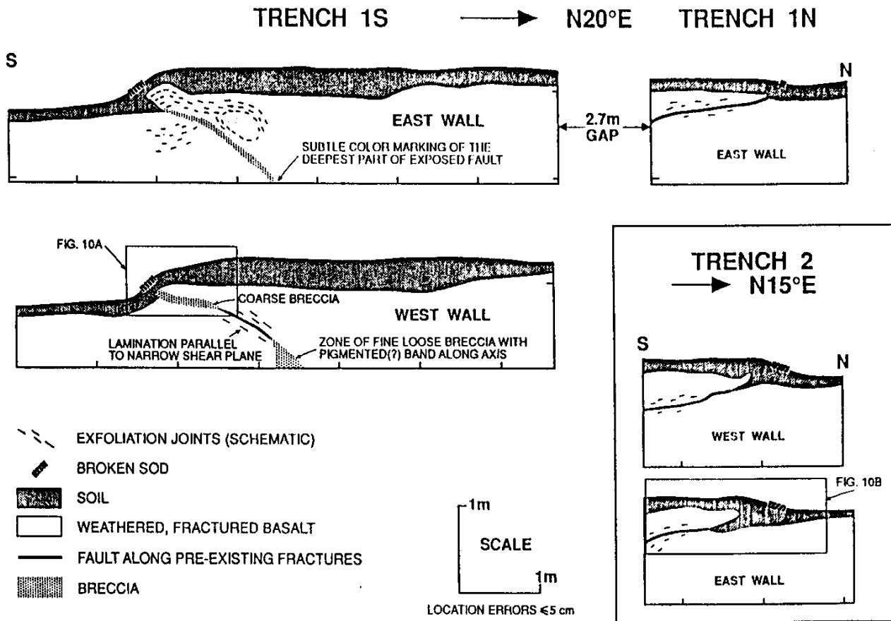
Figure 9. Maps of hand-excavated trenches across scarps associated with the mainshock rupture. All features shown (except exfoliation joints) were mapped to better than \pm 5 cm accuracy. Trenches 1 and 2 were along profiles 1 and 2 shown in Figure 5b. Soil was generally thicker, and weathering of basalt more pronounced, in the uplifted block between opposing thrusts. We did not have sufficient exposure to understand the significance of the loose breccia zone with subtle pigmentation at the bottom of the trench (see text).
