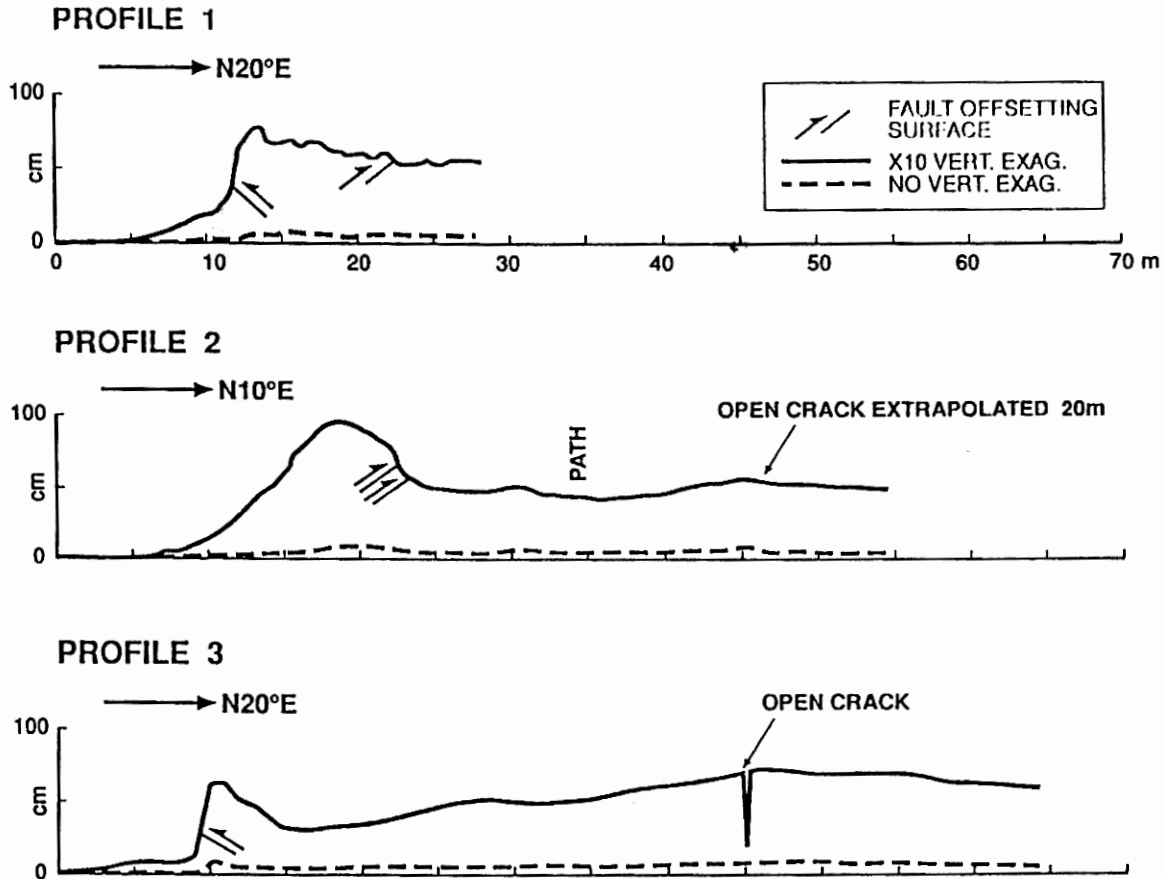
Figure 6. Topographic profiles across scarps. Profiles are located in Figure 5b.
