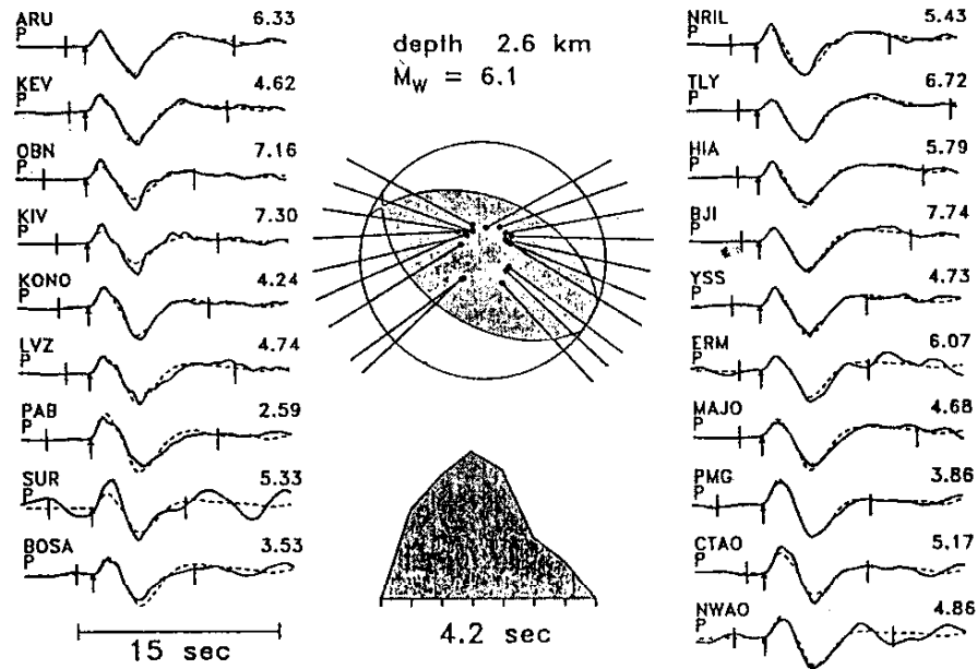
Figure 2. Moment tensor solution for the Killari mainshock in lower hemisphere, equal area projection. Solid circles mark ray paths crossing the hemisphere. The corresponding broadband teleseismic P waveforms are shown as solid lines, and the theoretical waveforms corresponding to the focal mechanism, source time function, and centroid depth are dashed. The southwest dipping nodal plain has strike, dip, rake of 126^\circ , 46^\circ , 100^\circ , respectively. The maximum amplitude (in microns) is to the right of each waveform pair. Small arrows show picked arrival times of the P phase, and vertical bars show the time window used in the inversion. The rate of moment release (arbitrary scale) and the duration (4.2 s; tick marks are 0.6 s apart) are shown by the normalized source time function below the focal mechanism.
