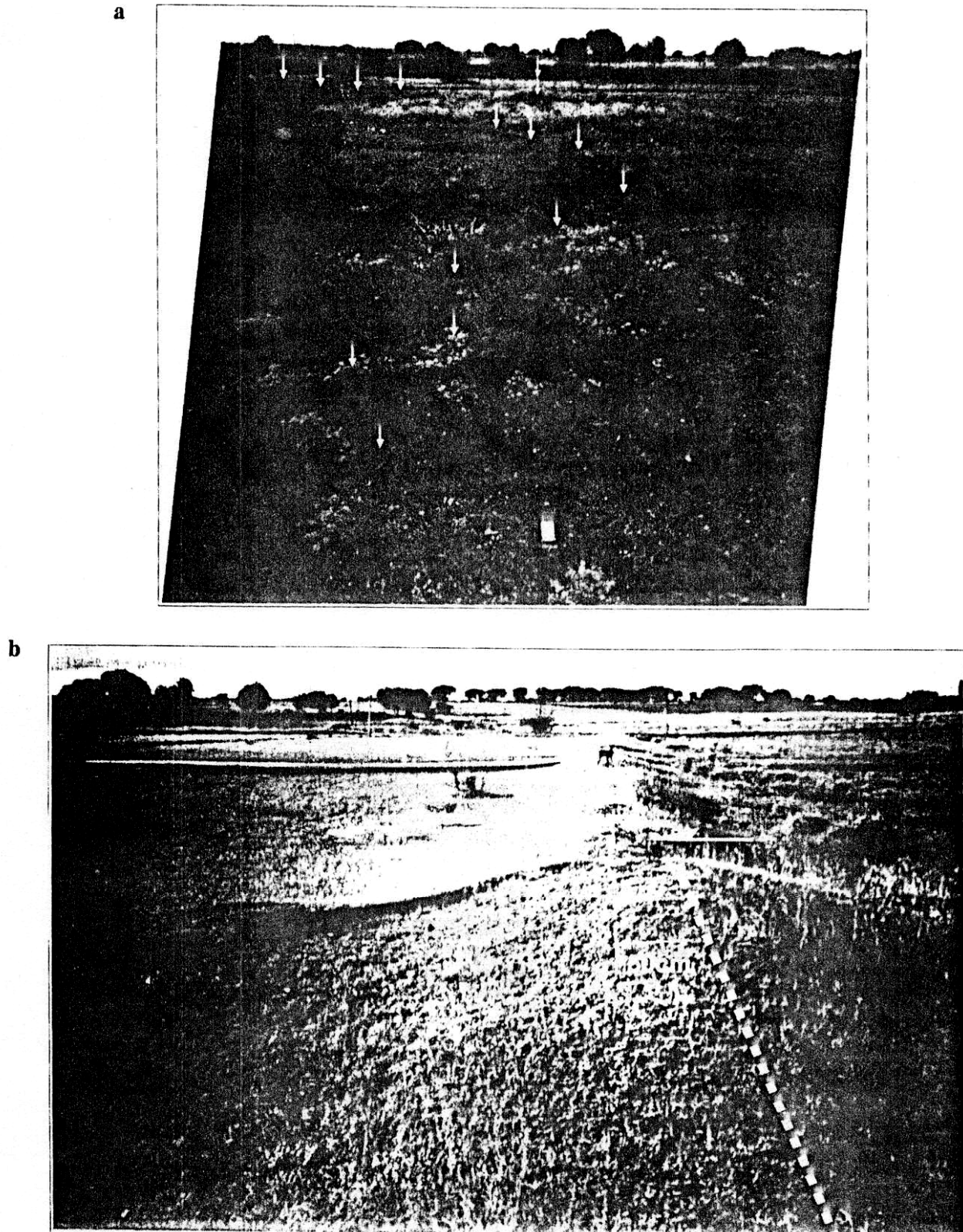
Figure 4. Photographs of scarps in the area of Figure 5b. (a) South facing scarp looking west from the site of trench 1 (marked by 10x6 cm compass on the ground). Tire tracks cross the scarp, which is marked by arrows. The double arrow marks the uplifted ground along profile 2 (Figure 5b). Note low relief in the background. (b) Northwest view along earthen berm (dashed line) offset 50 cm left-laterally by transfer fault T2 (Figure 5b).
