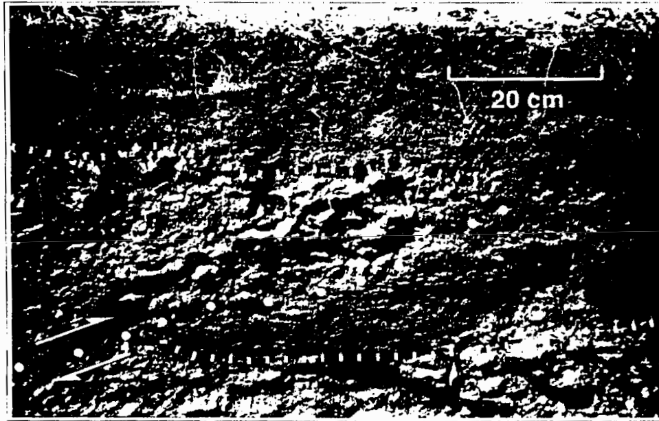
Figure 10c. Detailed view of the fault in Figure 10b, showing weathered basalt overriding soil by about 50 cm.
