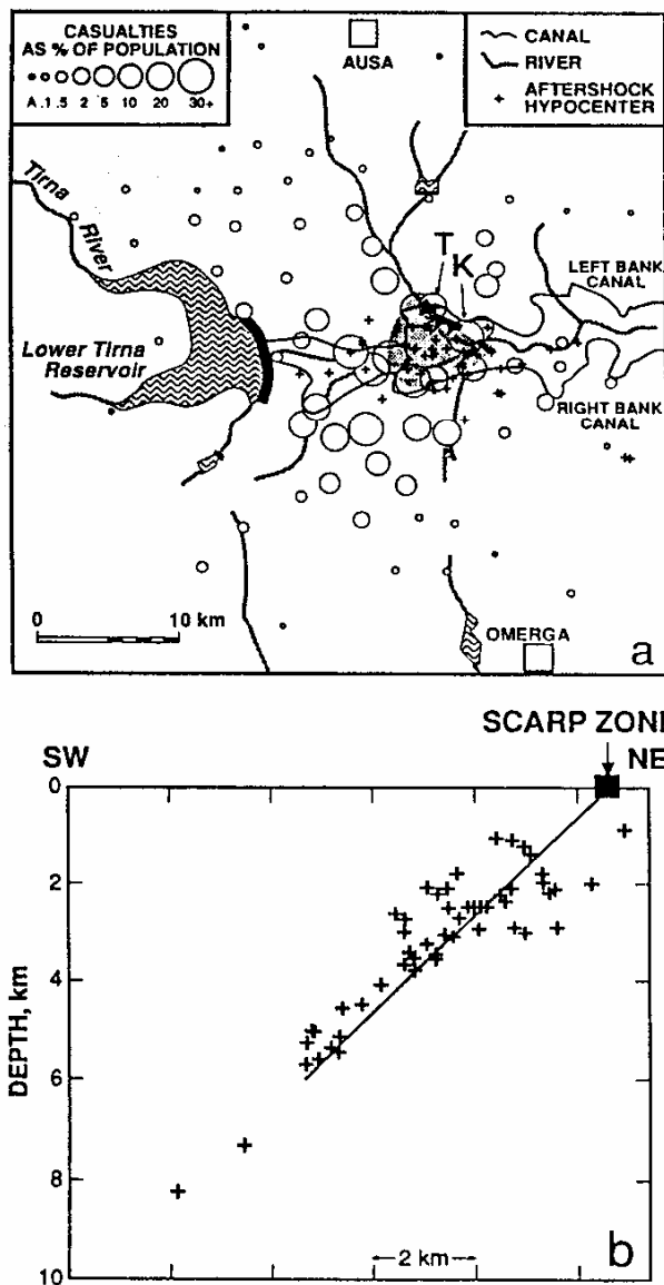
Figure 3. (a) Map and (b) vertical section (no vertical exaggeration) of data constraining the 1993 Killari mainshock rupture. The percentage of casualties in each village (Figure 3a; see text) delineates a 10-km-wide meizoseismal area, the surface rupture (heavy line; barbs on uplifted side of the buried fault) is west of Killari (K); near-surface rupture is inferred to warp the left-bank canal near Talni (T). Aftershock hypocenters [from Baumbach et al. , 1994] are clustered below the meizoseismal area on a plane dipping southwest and intersecting the surface rupture. The half ellipse in Figure 3a represents our best estimate of the location and size of the rupture (see text); it is centered about 10 km downstream of the lower Tirna dam (thick solid line).
